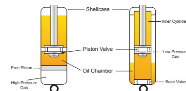
BILSTEIN'S MONOTUBE vs. COMPETITOR'S DUALTUBE
